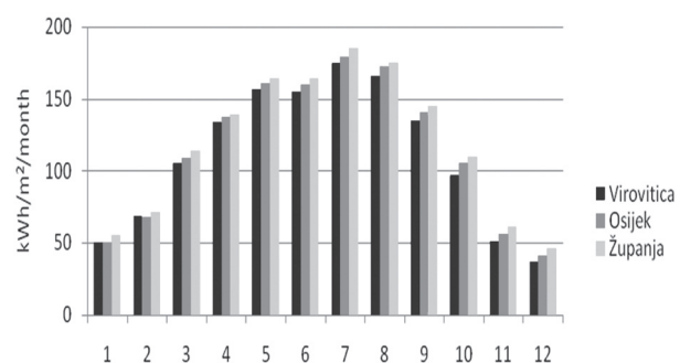
Fig. 8. Average monthly radiation data for Virovitica, Osijek and Zupanja (optimal angle) [5]
